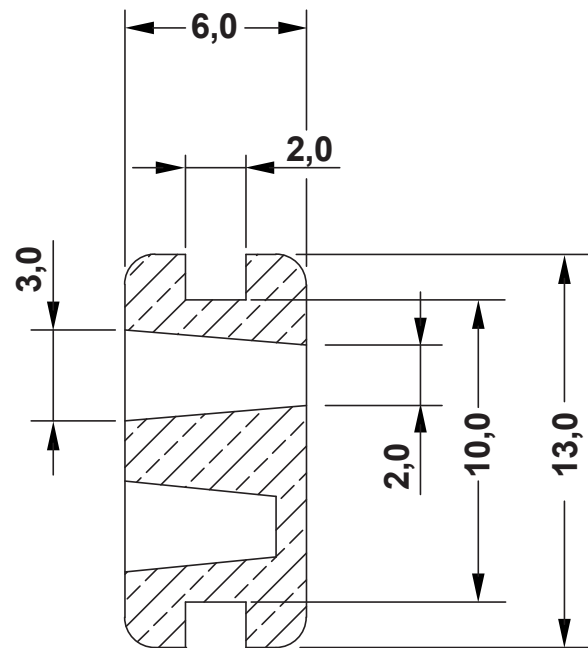
SECTION A - A CLOSED HOLE 1
