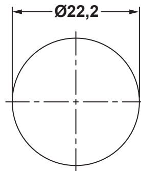
MOUNTING HOLE CHASSIS THICKNESS 0,8 - 3,3
