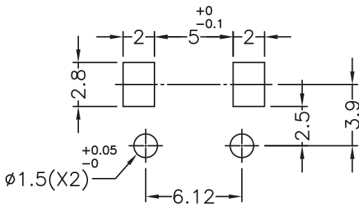
MOUNTING HOLES
